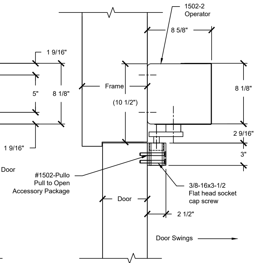
2 Section Head Detail: 1502-2
