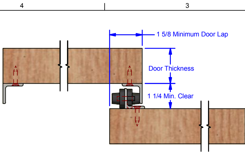
Plan View: Doors Full Closed
