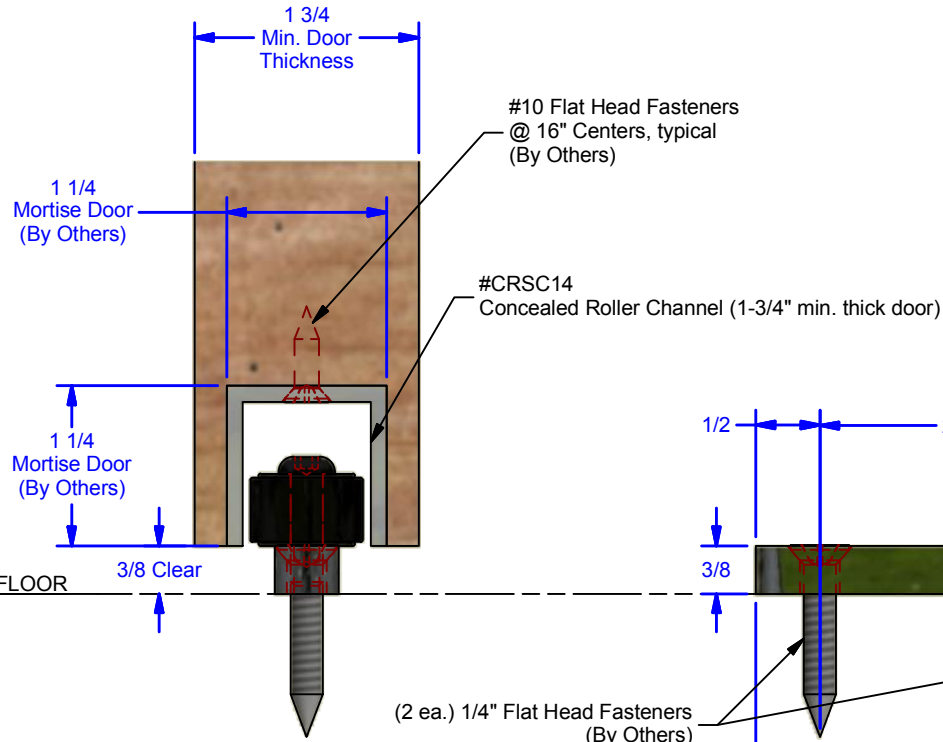
END VIEW
