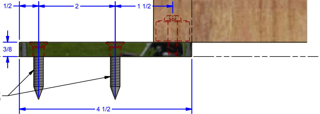
ELEVATION VIEW
