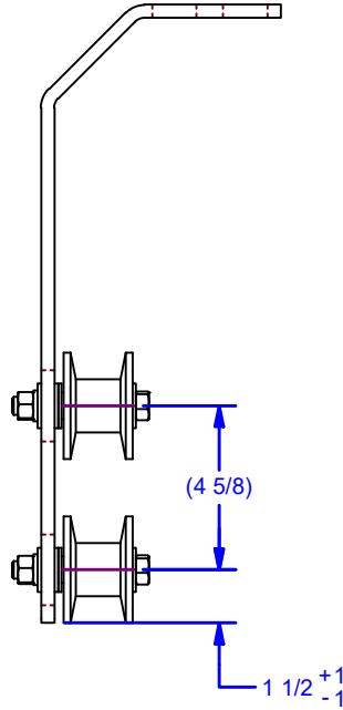
Double Wheel 1275P81 Double Chain Guide
