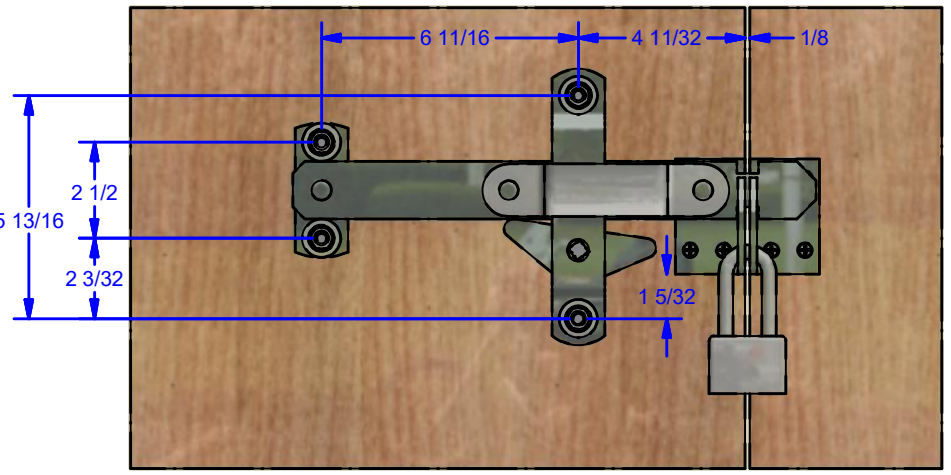
Non-Wall Elevation
