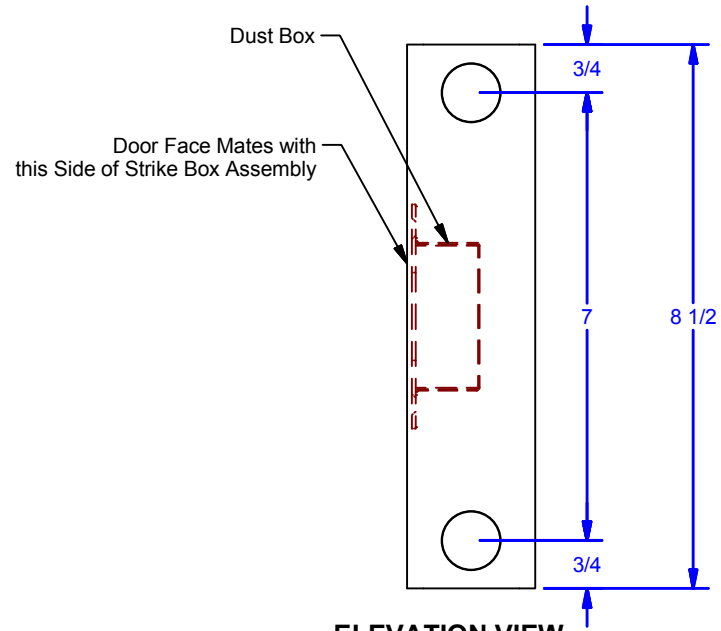
ELEVATION VIEW
