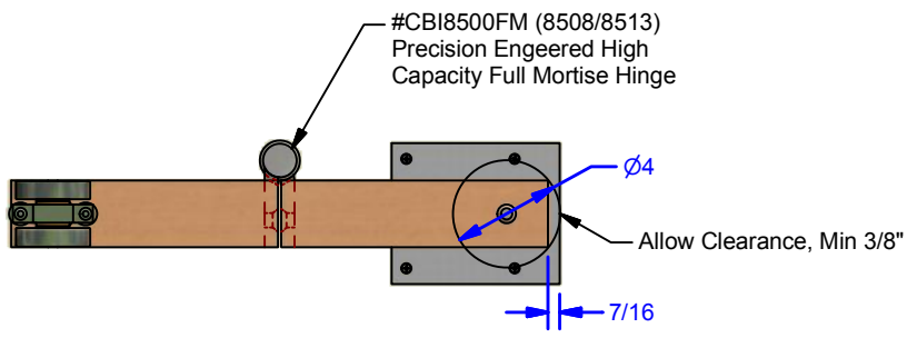
Plan View: Not Track
