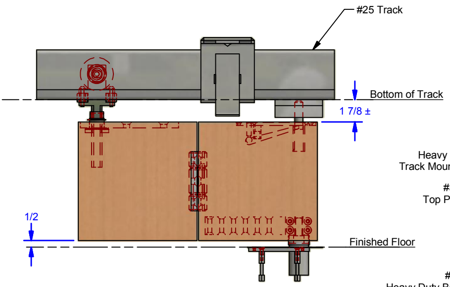
Exterior Elevation: Folding Out Option
