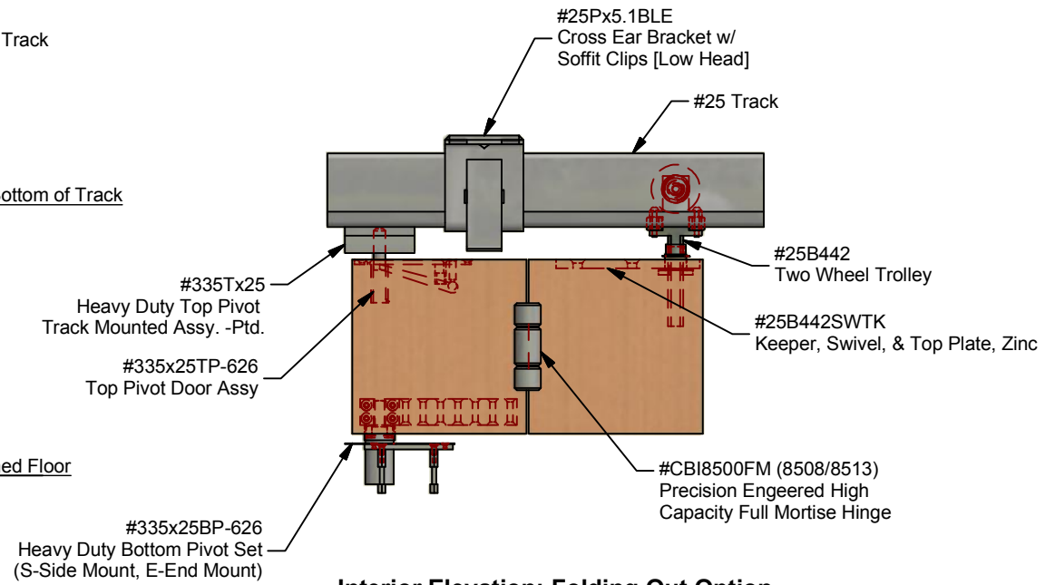
Interior Elevation: Folding Out Option
