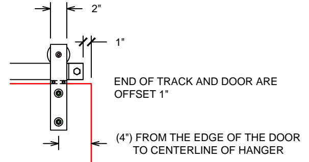
DETAIL A
