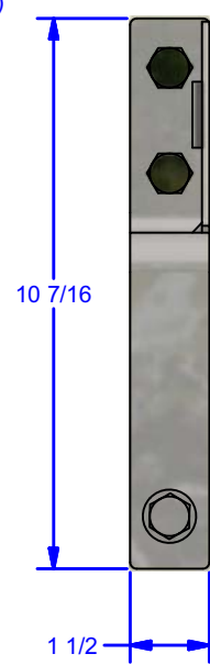
Elevation View of 43x22 Bracket
