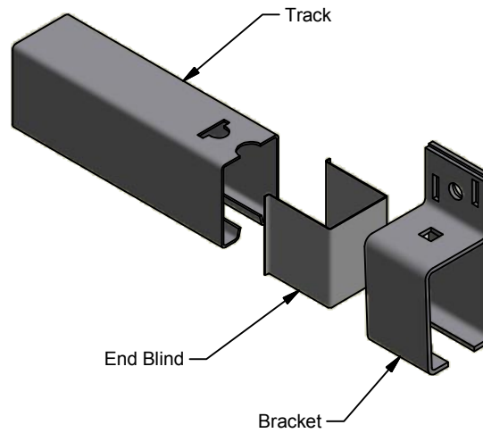
Disassembled View
