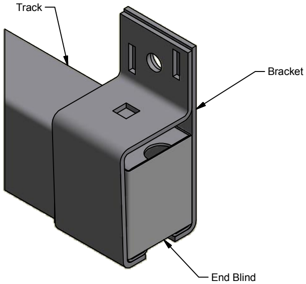
Assembled View
