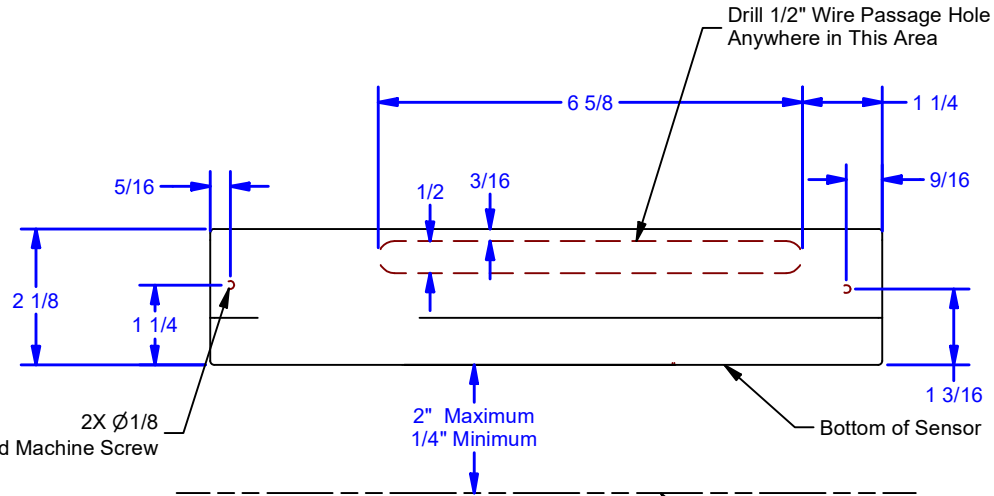
Front Elevation
