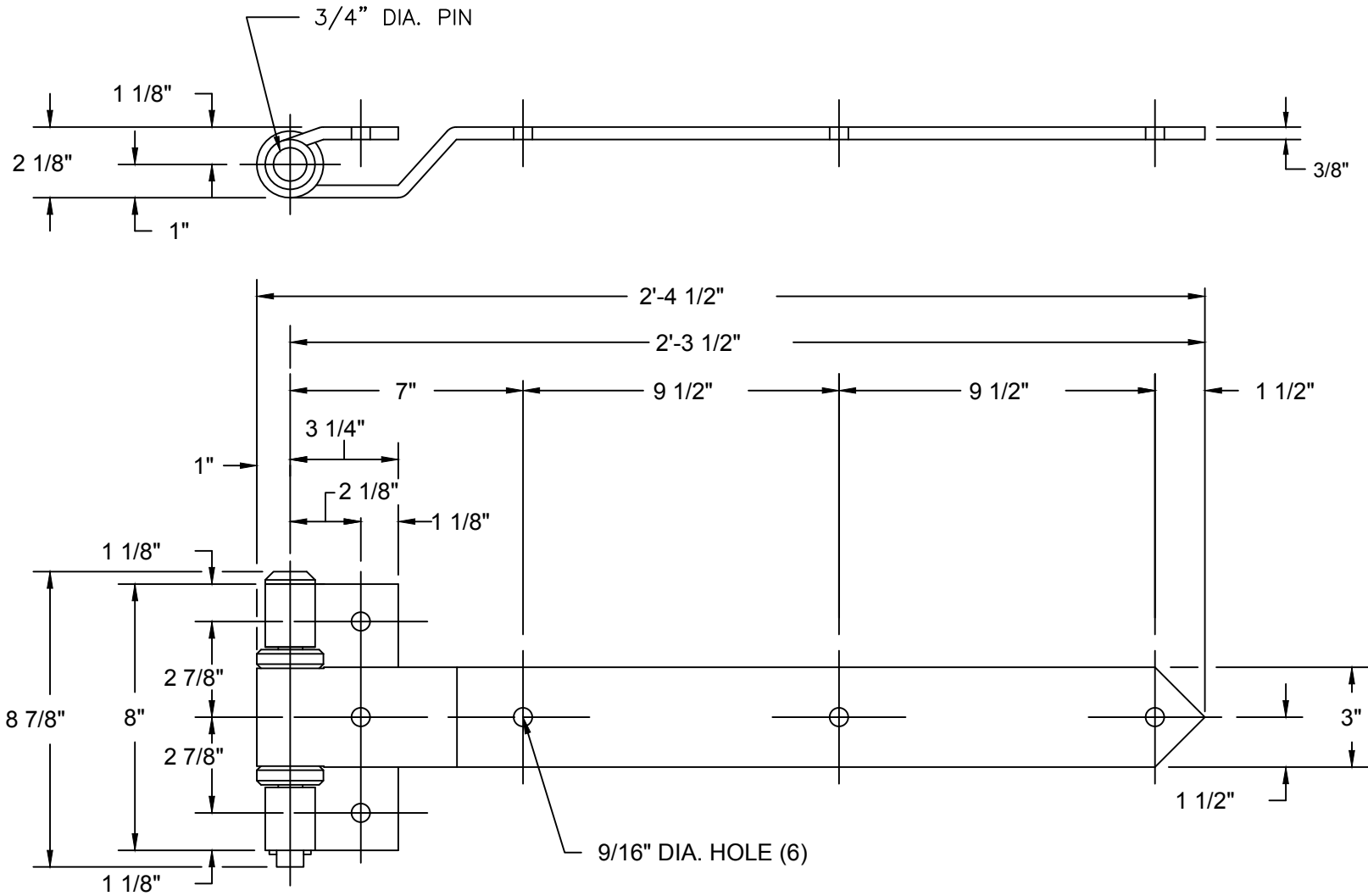
934.00323 BB-F HINGE 3/8 X 3
