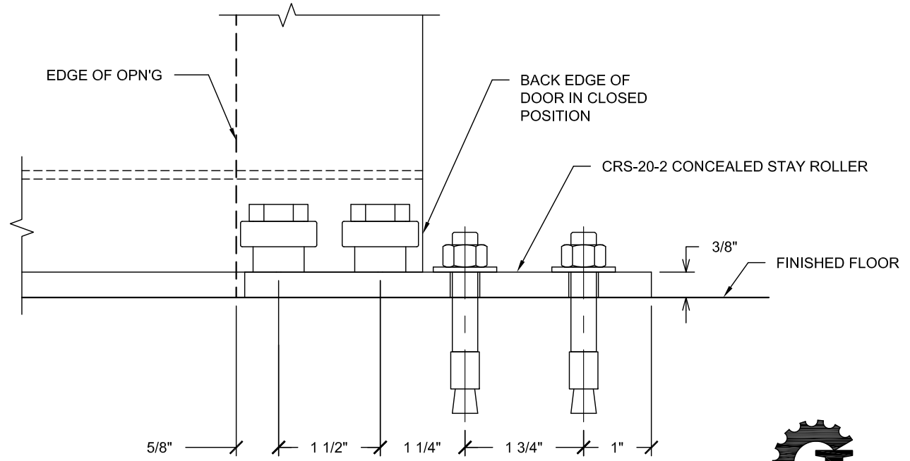
ELEVATION VIEW
