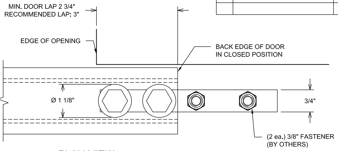
PLAN VIEW
