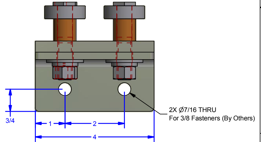
ELEVATION (NO DOOR)
