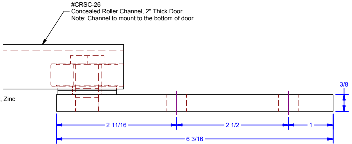
Elevation View
