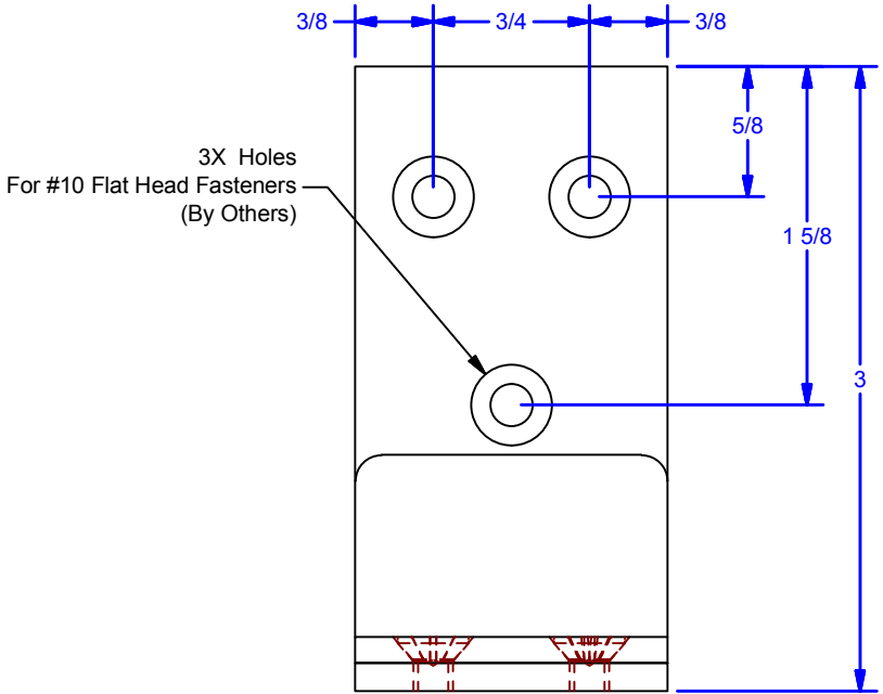
ELEV. VIEW
